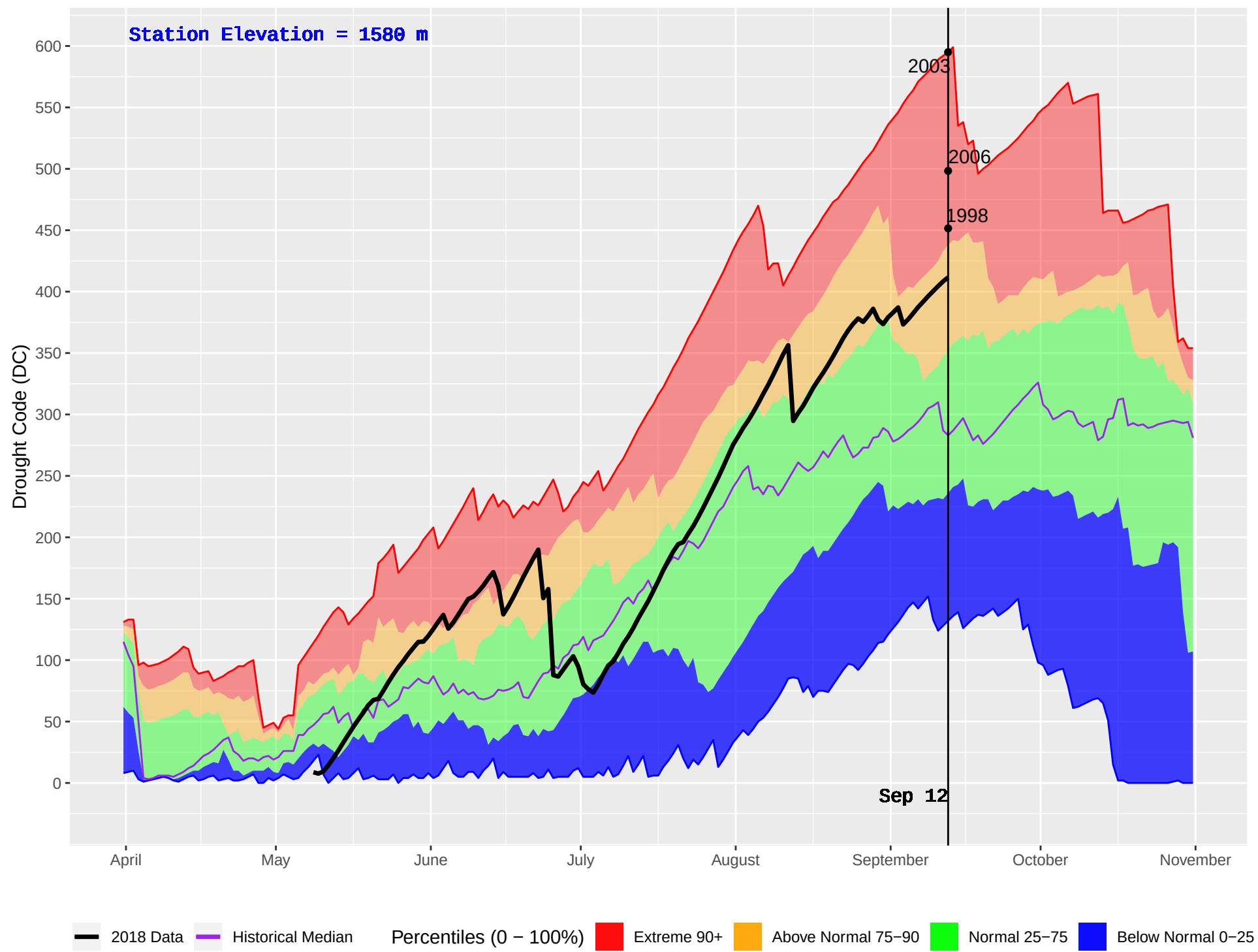
WINDY MOUNTAIN (244) : Historical (1989–2016) and Current (2018) Daily Drought Code (DC)
