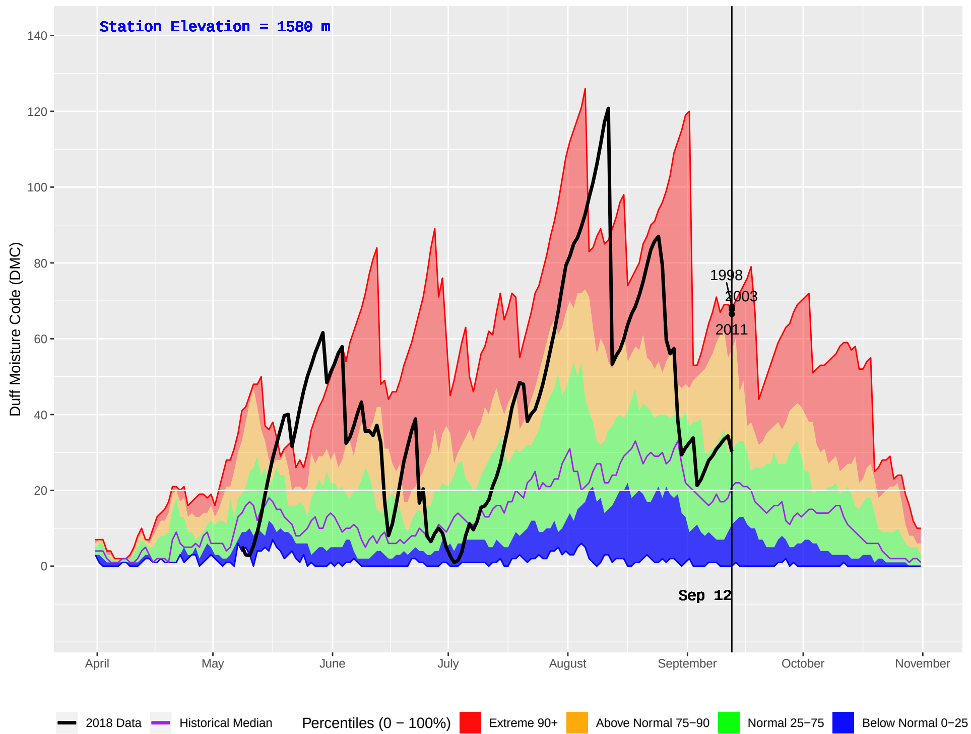
WINDY MOUNTAIN (244) : Historical (1989–2016) and Current (2018) Daily Duff Moisture Code (DMC)
