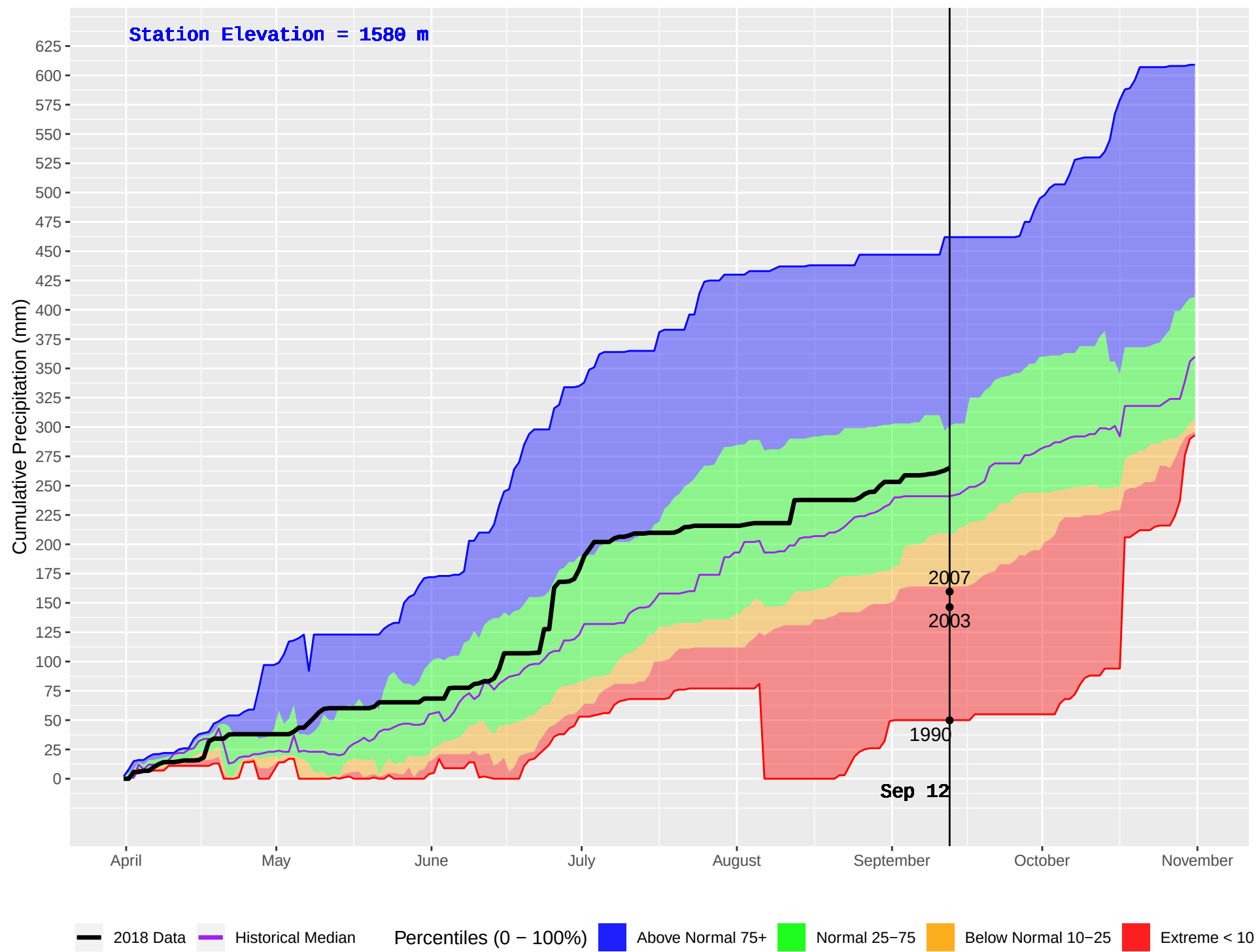
WINDY MOUNTAIN (244) : Historical (1989–2016) and Current (2018) Daily Cumulative Precipitation
