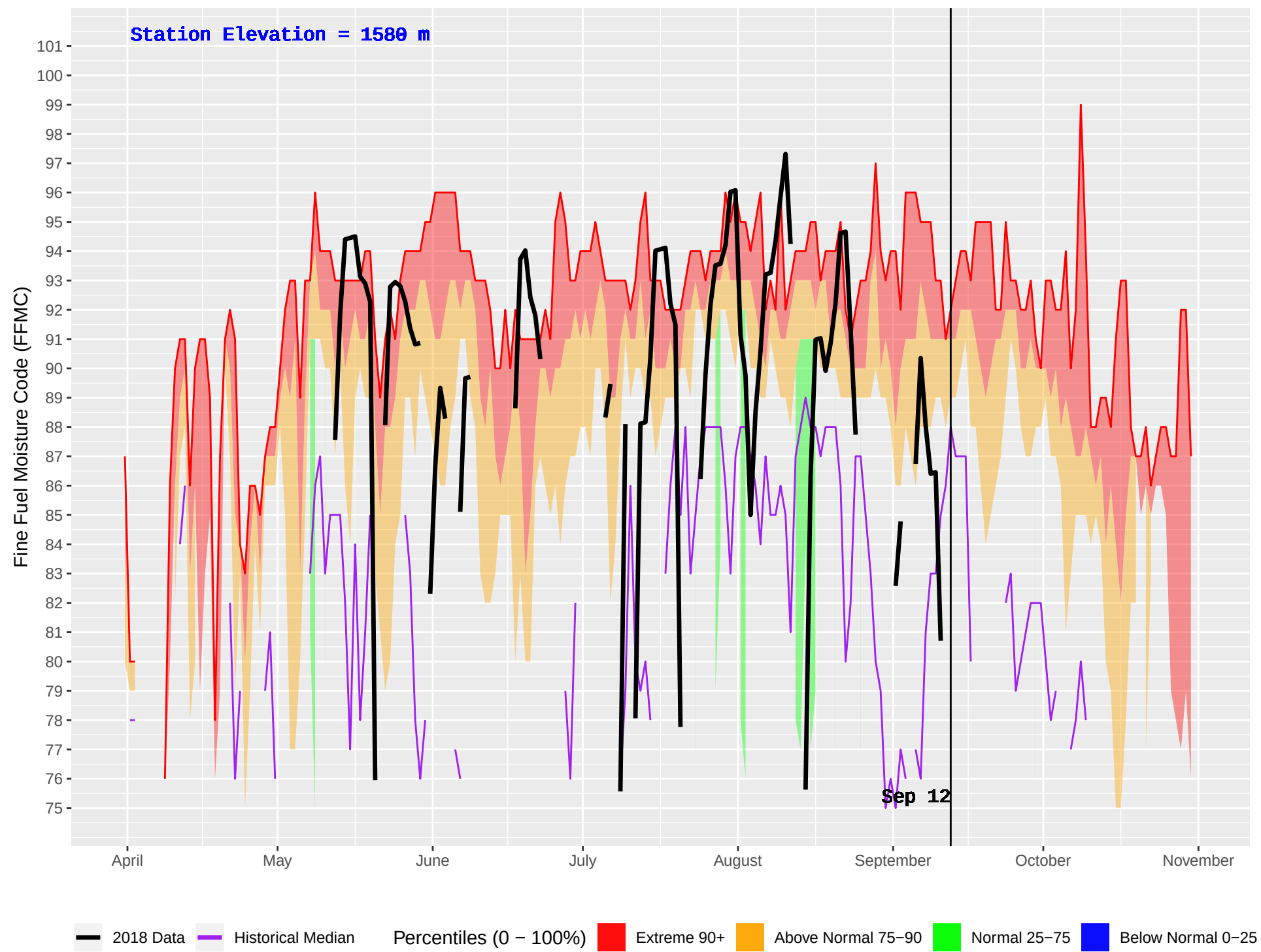
WINDY MOUNTAIN (244) : Historical (1989–2016) and Current (2018) Daily Fine Fuel Moisture Code (FFMC)
