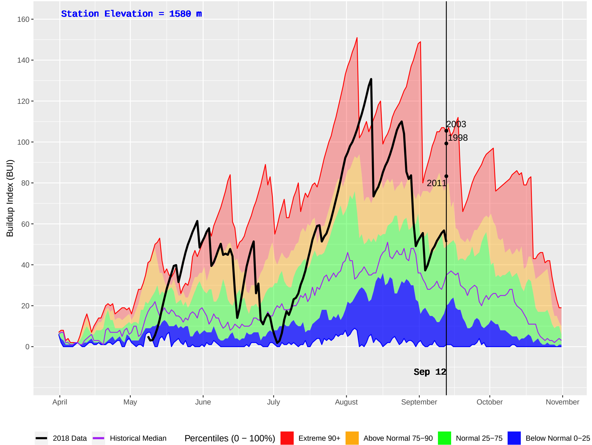
WINDY MOUNTAIN (244) : Historical (1989–2016) and Current (2018) Daily Buildup Index (BUI)
