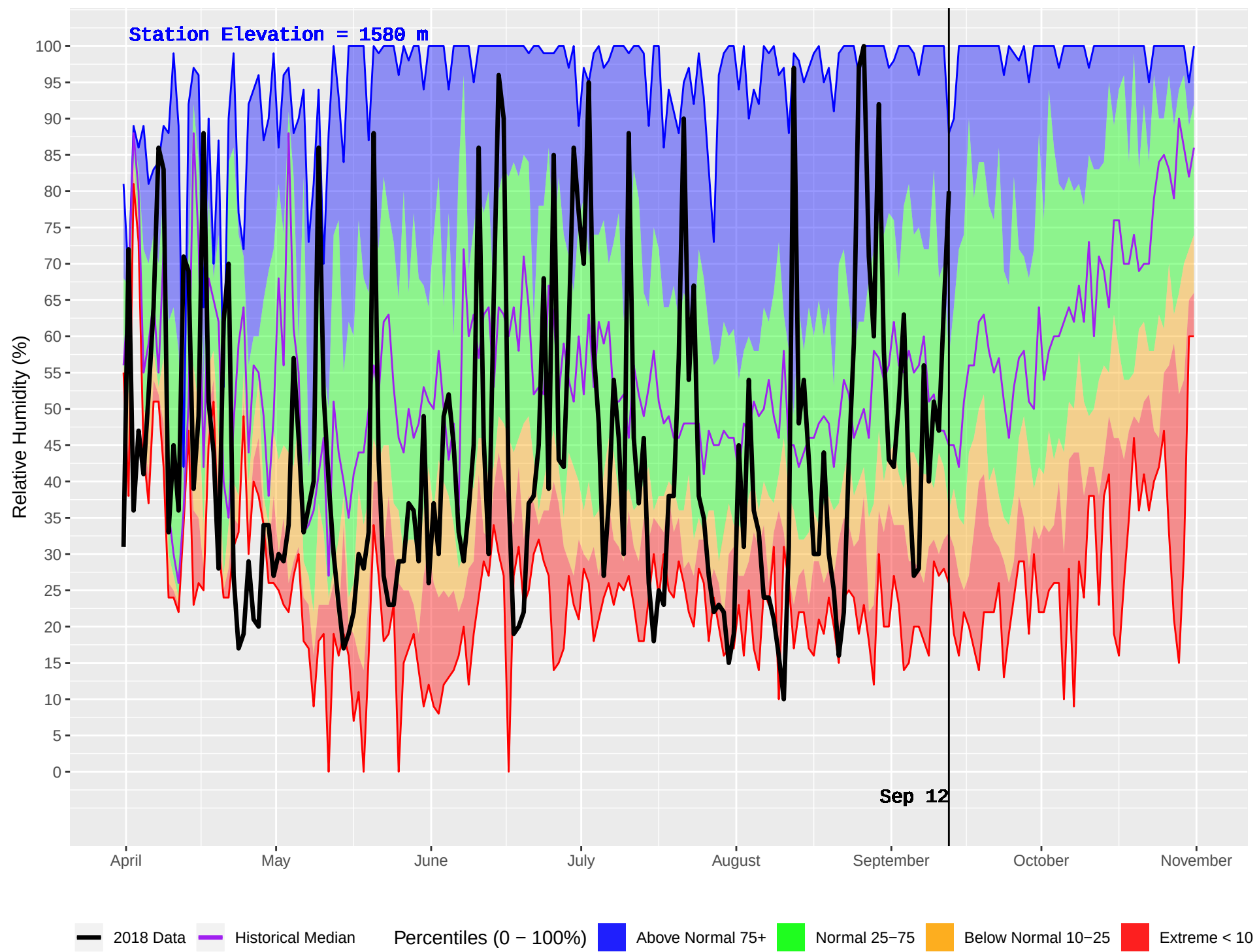
WINDY MOUNTAIN (244) : Historical (1989–2016) and Current (2018) Daily Relative Humidity
